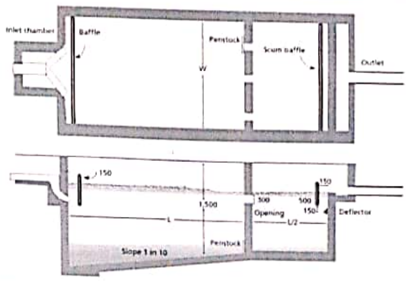
All measurements in millimetres (mm) Source: Manual on Sewerage and Sewage Treatment - Part A, Engineering, CPWD, 2012
